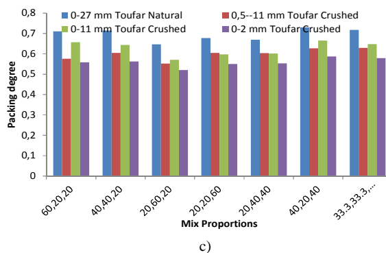
Fig. 13 Comparison between particle packing for natural and crushed aggregate and the same mix proportions, (a) from experimental tests, (b) from 4C program and (c) from Toufar's model
