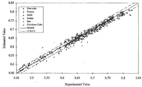
Fig. 16 Experimental packing degree versus estimated packing [3]
