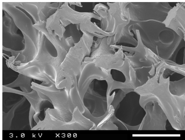
Fig. 1-b SEM image of PVF sponge immersed in dextran solution
