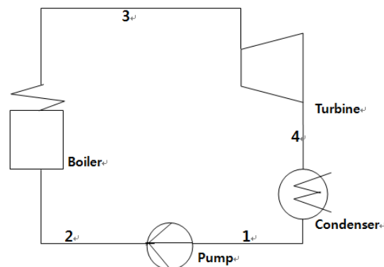
Fig. 1 Rankine Cycle
