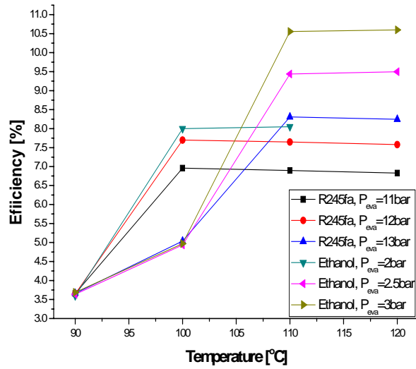
Fig.8 Cycle efficiency of LT loop with ethanol and R-245fa
