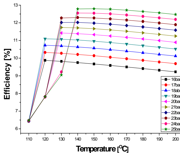
Fig. 10 Cycle efficiency of LT loop with ethanol
