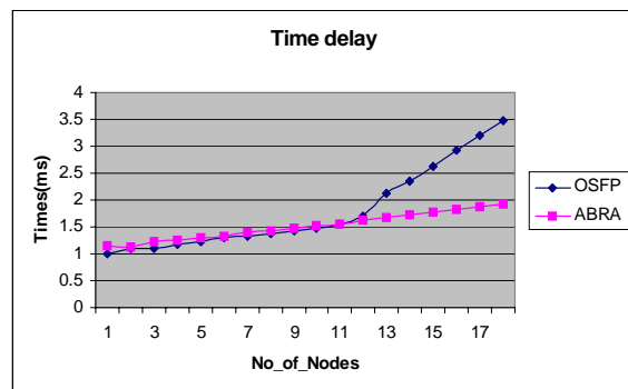
Fig. 4 a time delay at no of nodes from 3 to 20 and 5 agents
