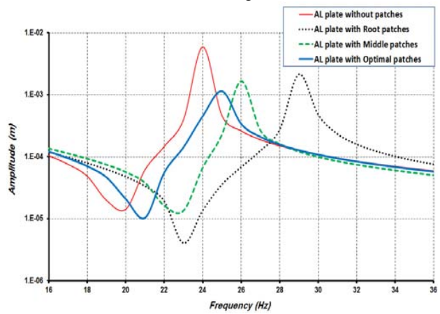
Second bending mode
