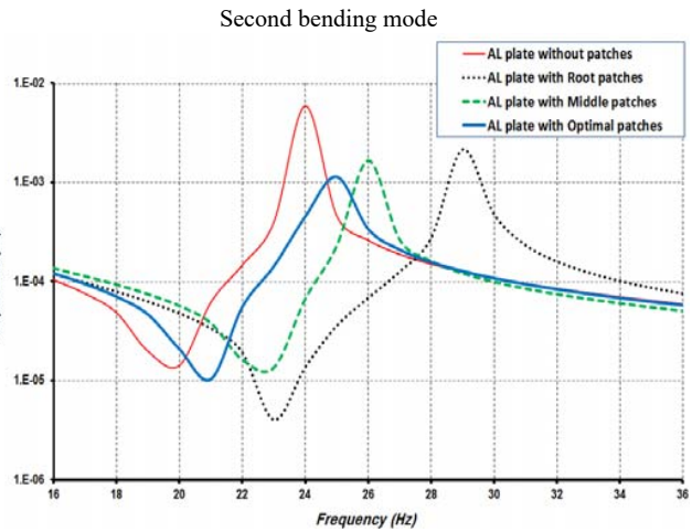
Fig. 5 The plate amplitude FRF at different patch locations: (a) First bending mode, (b) Second bending mode
