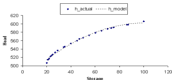
Fig. 1 Storage (million cubic meters) against water surface height (meter) in series 1 and real state (series 2)
