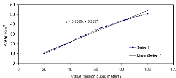
Fig. 2 Linear system of surface volume-area relations
