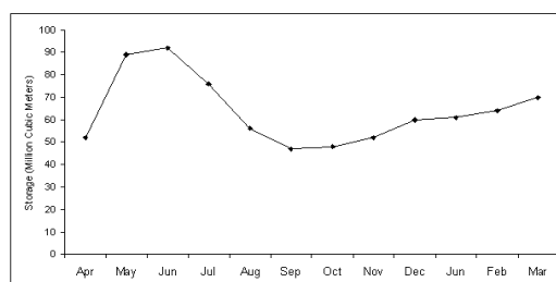
Fig. 3 Curve of reservoir exploitation of Meijaran Dam
