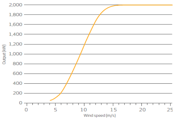
Fig. 1 Power curve of a WTG
