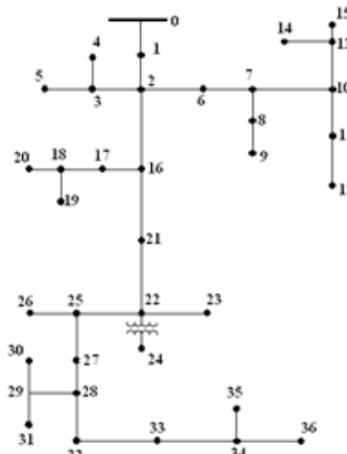
Fig. 3 Renumbered IEEE 37- node feeder
