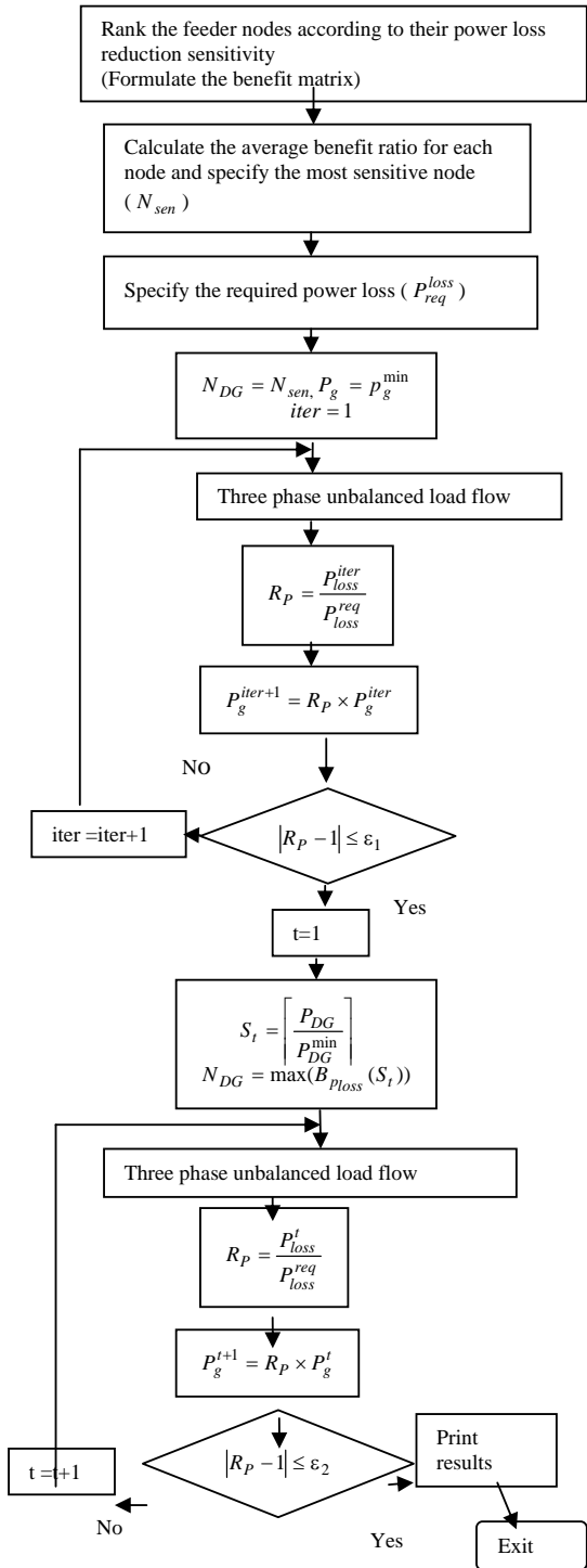
Fig. 2 Flow chart of the proposed heuristic technique
