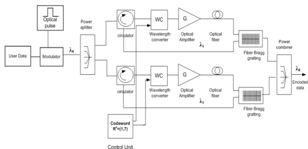
Fig. 3 Tunable optical decoder architecture
