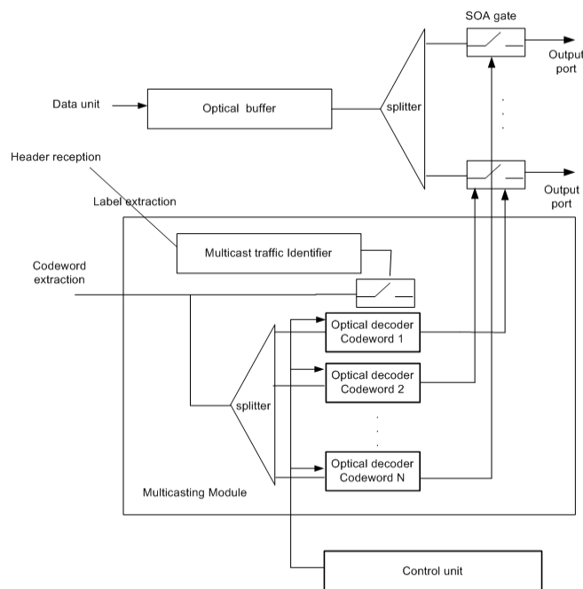
Fig. 2 Optical multicast core node design
