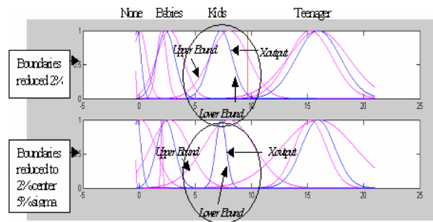
Fig. 8 Illustration of the Lower and Upper boundary for the MFs
