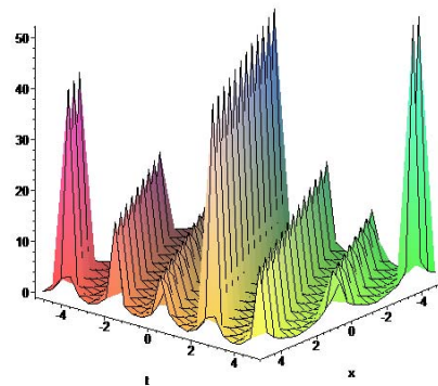
Fig. 1. The periodic solution u_1(x,t) which is a periodic wave for k = 2, A = 3, B = 1
