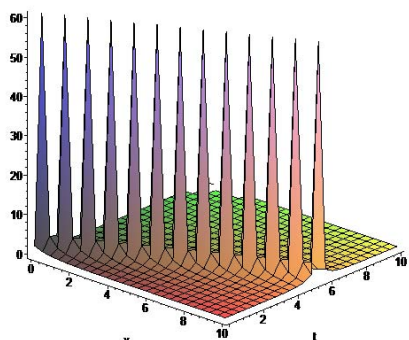
Fig. 2. The traveling solution of the field u_{10}(x, t) for k = 1, A = 2, B = 3
