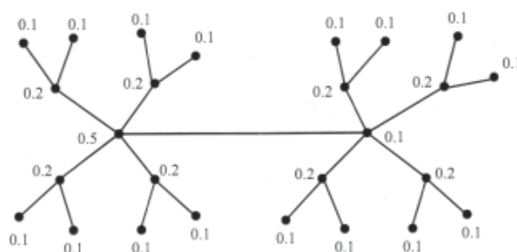
Fig.2 Fuzzy graph G
