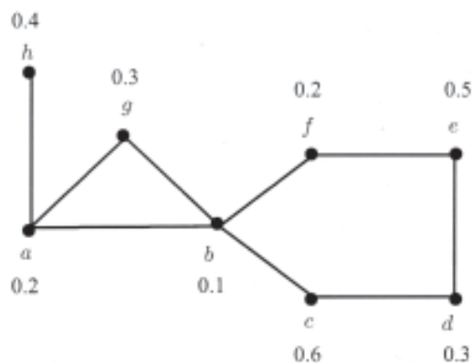
Fig.1 Fuzzy graph G
