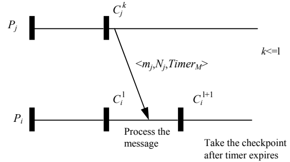
Fig. 3 Case 2 ( N_j \leq N_i )
