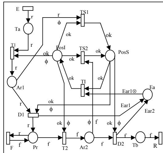
Fig. 3 ECATNet model of the cell
