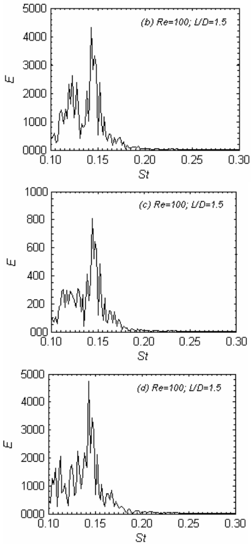
Fig. 9 Fourier spectrum analysis of lift coefficient for spacing ratio 1.5 (a) Cylinder1, (b) Cylinder2, (c) Cylinder3, (d) Cylinder4
