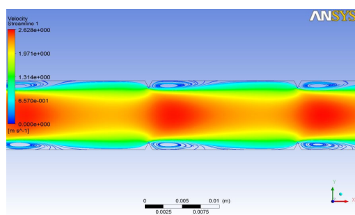
(C) Re=40000
