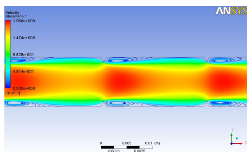
(B) Re=30000
