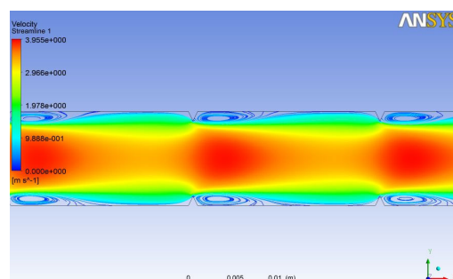
(E) Re=60000
