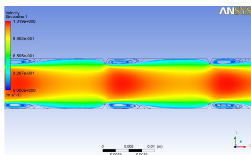
(A) Re=20000
