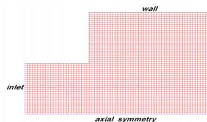
Fig. 2 Numerical grid of the computational domain at inlet
