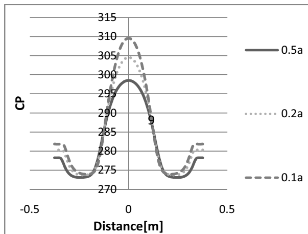
Fig. 17 Dimensionless normal pressure CP, for three different curved profiles – local distribution
