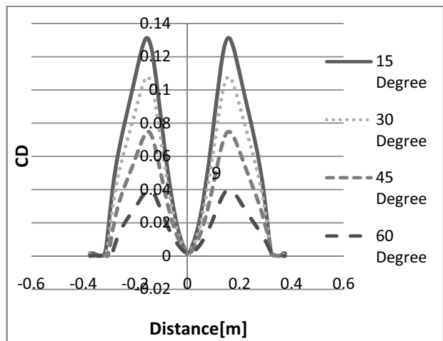
Fig. 14 Dimensionless shear stress CD, for four different nozzle angle – local distribution
