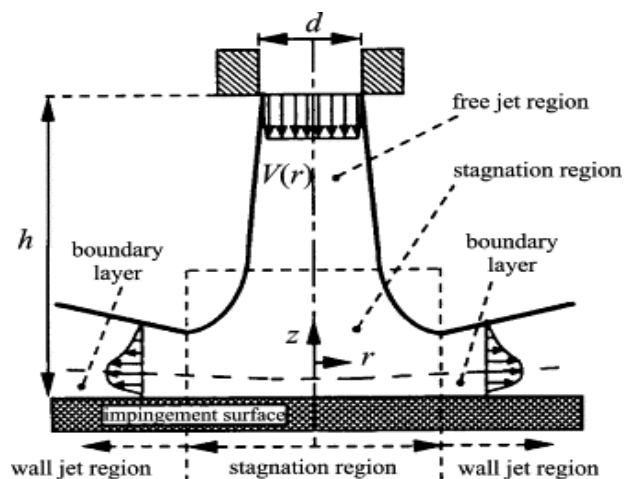
Fig. 1 Three different region of flow in jet impingement on a wall, nozzle diameter d and distance h [9]
