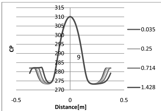
Fig. 9 Dimensionless normal pressure CP- for four different impingement wall velocities-local distribution
