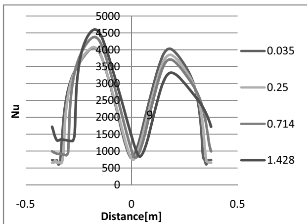
Fig. 8 Dimensionless Heat transfer coefficient Nu for four different impingement wall velocities - local distribution
