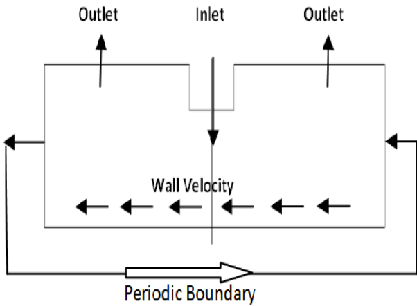
Fig. 7 Model with moving surface
