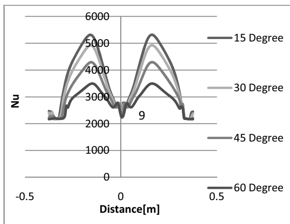
Fig. 12 Dimensionless heat transfer coefficient Nu for four different nozzle angles – local distribution
