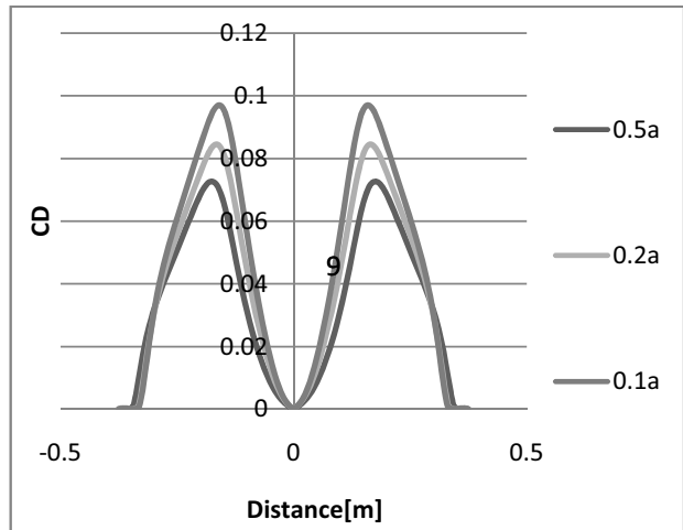
Fig. 18 Dimensionless shear stress CD, for three different curved profiles – local distribution
