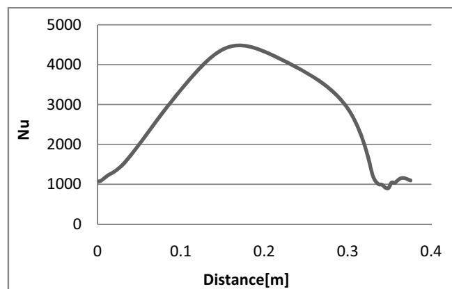
Fig. 4 Dimensionless heat transfer coefficient Nu – local variation
