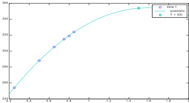
Fig. 3 Value of heat transfer coefficient for different mesh sizes
