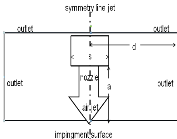
Fig. 2 Model Geometry
