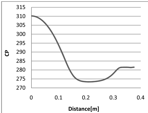
Fig. 5 Dimensionless normal pressure CP – local distribution
