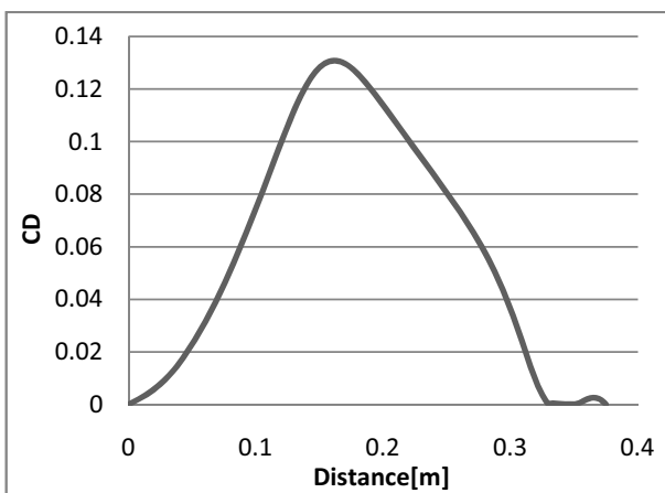
Fig. 6 Dimensionless shear stress CD – local distribution
