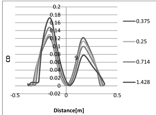
Fig. 10 Dimensionless shear stress CD, for four different impingement wall velocities-local distributions
