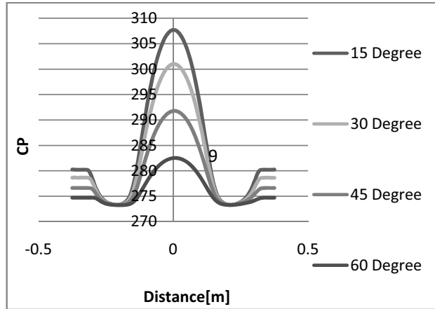
Fig. 13 Dimensionless normal pressure CP for four different nozzle angle – local distribution
