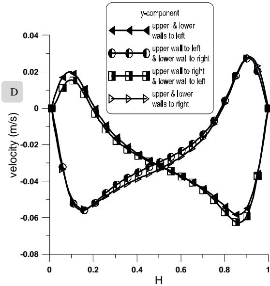
Fig. 5 Velocities distributions for cases (9-16)
