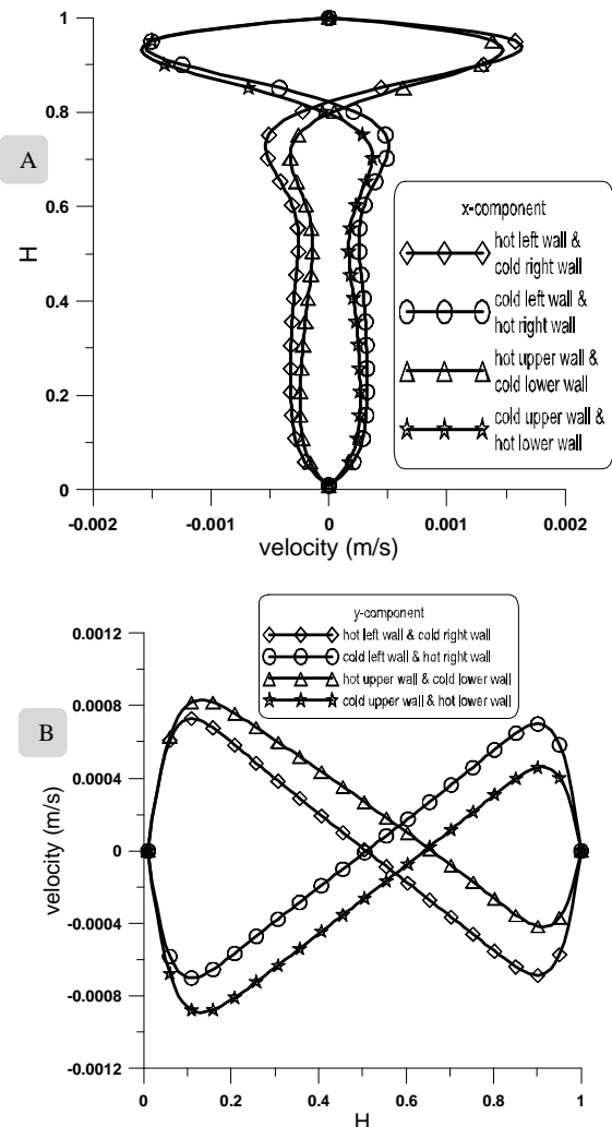
Fig. 8 Velocities distributions for cases (22-25)
