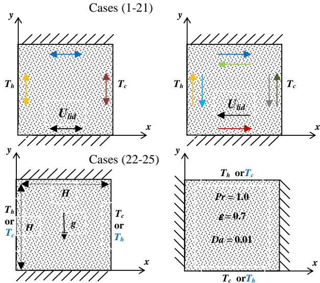
Fig. 1 Schematic diagram for the problem, physical models and cases with the wall boundary constraints and the coordinate axes.
