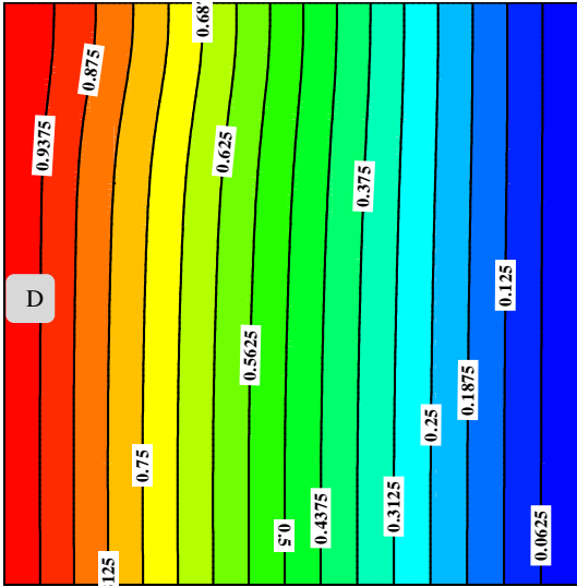
Fig. 7 Velocity vector and temperature contour for case(22).
