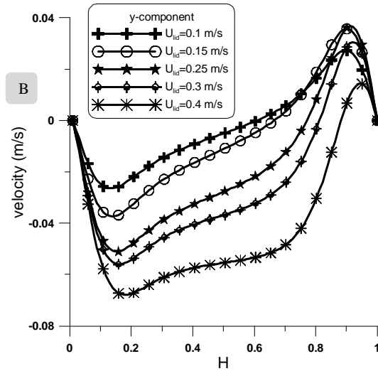
Fig. 6 Velocities distributions for cases (17-21)
