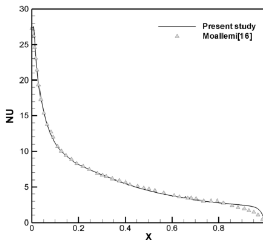
Fig. 4 Nusselt local on Lid-driven wall
