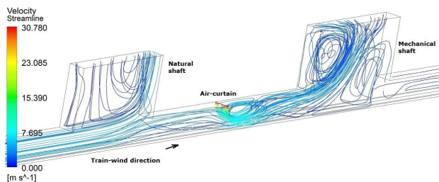
b) Velocity of the air-curtain is 30 m/s
