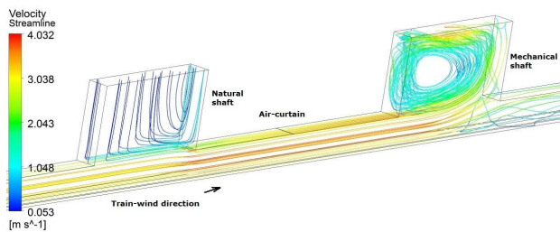
a) Velocity of the air-curtain is 0 m/s
