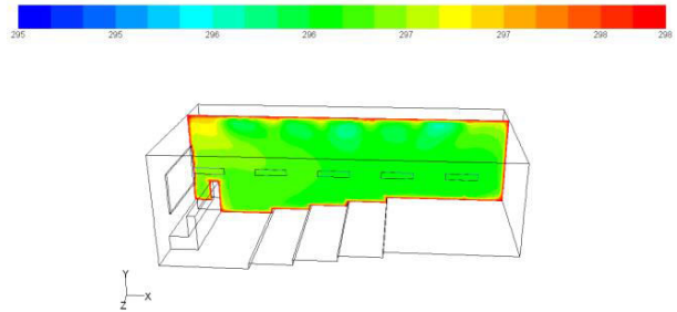
Fig. 14 (Case 2) Temperature contours (K), vertical plane at Z=1.5 m
