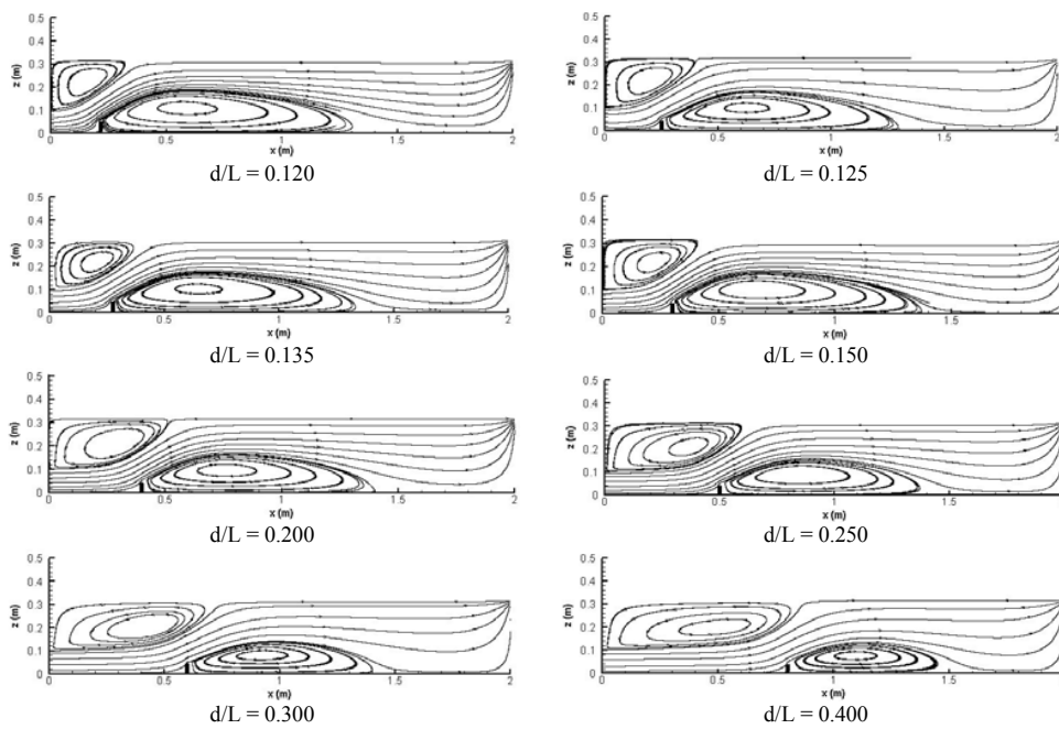
Fig. 3 Streamlines of different baffle positions in sedimentation tank
