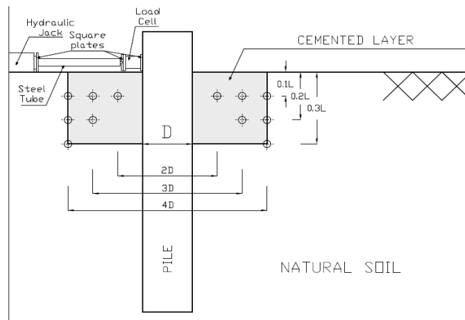
Fig. 3 Schematic view of insitu tests [8]
