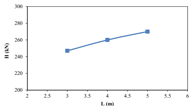
Fig. 7 Evaluation of lateral bearing capacity of piles with pile length
