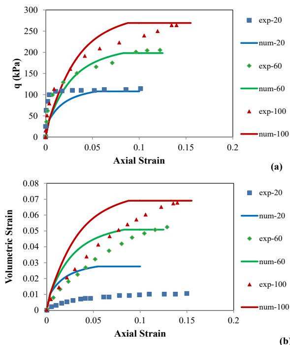
Fig. 1 Experimental results and numerical modeling of triaxial test on natural soil (a) Deviatoric stress stress-Axial strain, (b) Volumetric strain-Axial strain[8]
