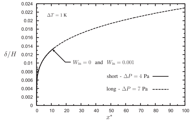
Fig. 2 Film thickness
