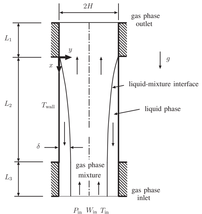
Fig. 1 Reflux condensation-model domain
