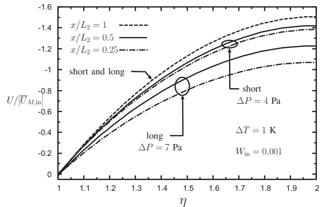
Fig. 3 Velocity profiles
