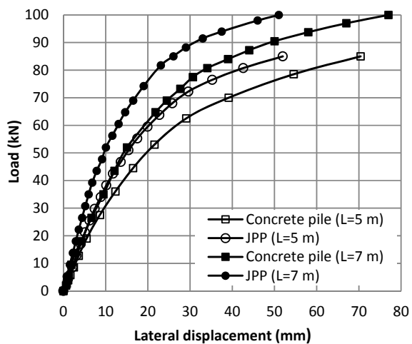
Fig. 4 Lateral load-displacement behavior for considered piles
