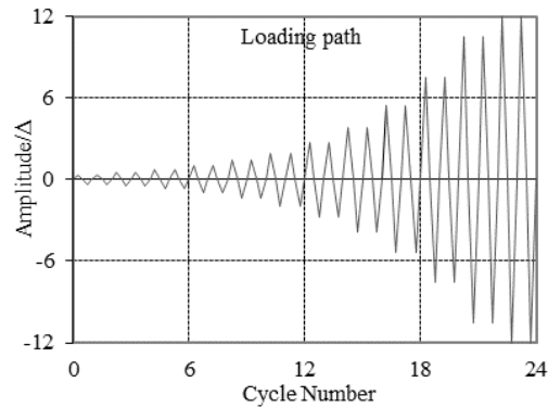
Fig. 5 CUREE reversed cyclic test protocol
