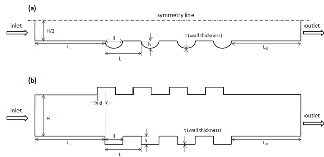
Fig. 1 Channel geometry (a) symmetric configuration with arc-shaped grooves, (b) staggered configuration with rectangular grooves
