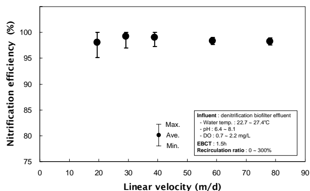
Fig. 2 Effet of the linear velocity on the nitrification efficiency
