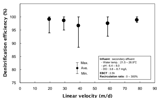
Fig. 1 Effet of the linear velocity on the denitrification efficiency
