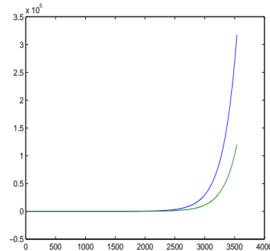
Fig. 5. Behavior of the state component of the switched neutral subsystem1.
