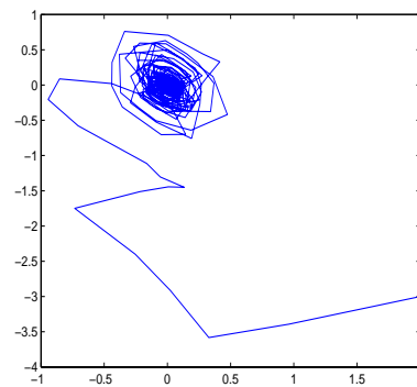
Fig. 4. The phase map of the switched neutral systems.
