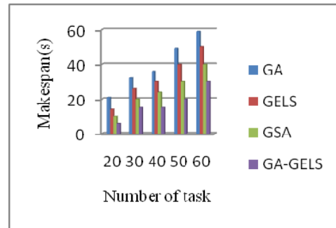
Fig. 3 Comparison of Makespan
