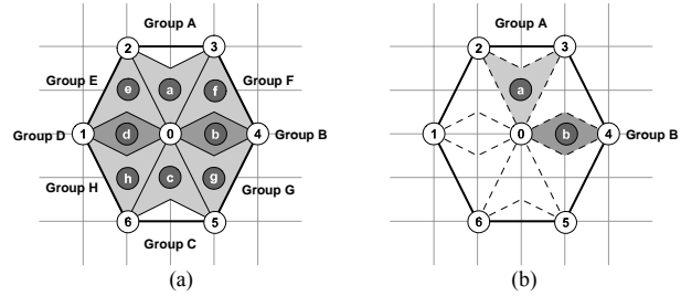
Fig. 5 (a) The new grouping for the hexagonal search pattern based on minimizing mean internal distance (MID). The eight inner points are separated into 2 sets by the MID value – Set-1: \{a, c, e, f, g, h\} and Set-2: \{b, d\} . (b) Point ‘a’ and ‘b’ are searched finally, because group A and group B have the smallest normalized group distortion in the corresponding set
