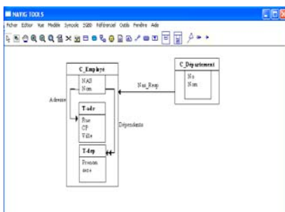
Fig.7 Navigational Model
