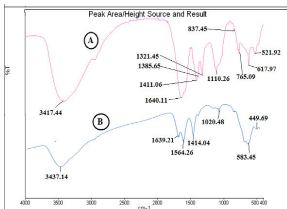
Fig. 2 (A) FTIR spectrum of dried aqueous extract of Datura innoxia leaves. (B) FTIR spectrum of synthesized \text{Fe}_3\text{O}_4 magnetic nanoparticles
