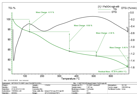
Fig. 3 Thermogravimetric analysis (TGA) results of magnetic nanoparticles
