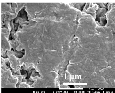
Fig. 4 SEM image for \text{Na}_{0.1}\text{V}_2\text{O}_5.n\text{H}_2\text{O} nanocrystalline film
