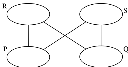
Fig. 6 Diagram representing the vertex partitioning of K_{n,n} .
