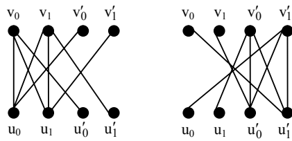
Fig. 9 A 4-sun decomposition of K_{4,4}
