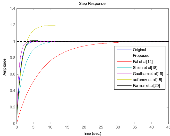
Fig. 1 Comparison of Step Responses of Original, Proposed and Other Existing Reduced Models of SISO System
