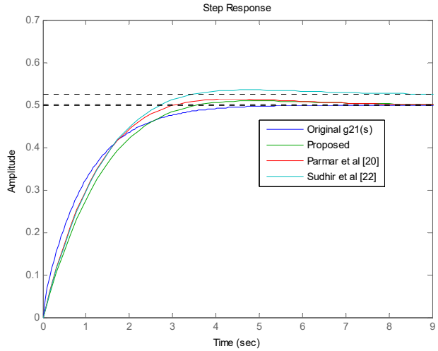
Fig. 4 Comparison of Step Responses of G_{21}(s) , Proposed Reduced and Other Existing Methods
