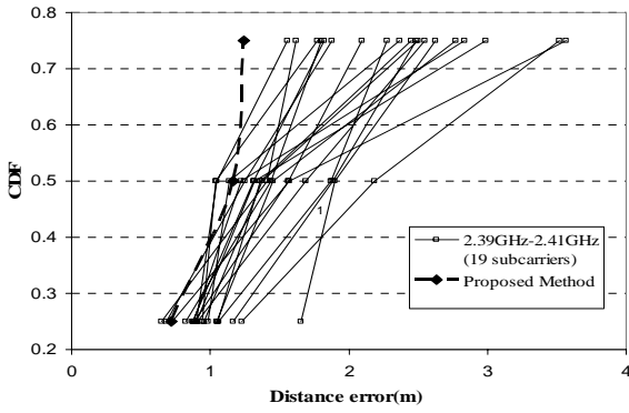
Fig. 9 Comparison of our proposed DOA location estimation method (multiple subcarriers) to other 19 subcarriers (narrowband) at Gymnasium hall
