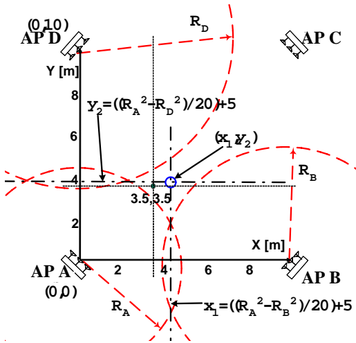
Fig. 7 RSSI-based estimation for AP AB-DA
