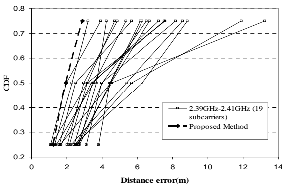
Fig. 10 Comparison of our proposed DOA location estimation method (multiple subcarriers) to other 19 subcarriers (narrowband) at seminar room
