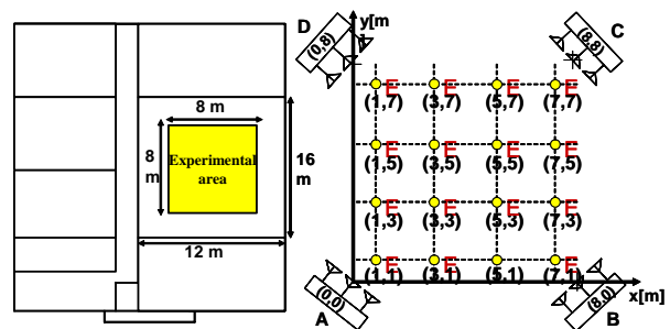
Fig. 4 Typical LOS office environment and experimental setup.
