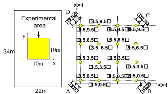
Fig. 3 The gymnasium layout and 4 APs with 16 location points.
