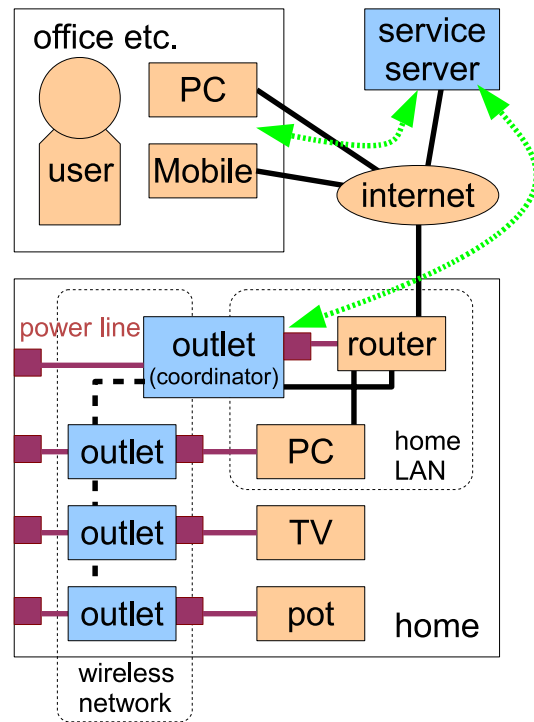
Fig. 1. Network configuration of proposed system
