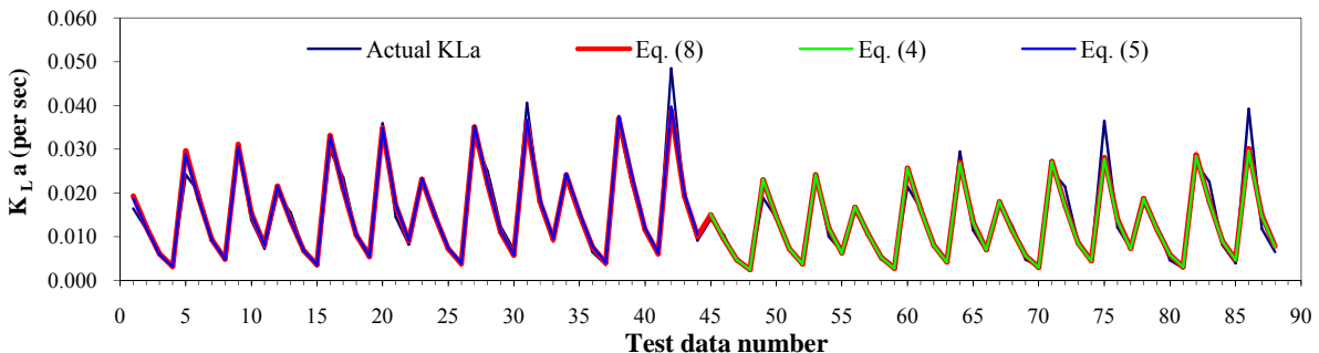
Fig. 5 Variation in predicted values by (8) in comparison to (4), (5) and the actual values of overall oxygen transfer coefficient at standard condition ( K_{L,a} ) by vertical and inclined multiple plunging jets
