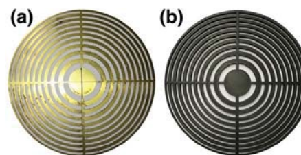
Fig. 4 Implemented FZP lenses. Material used for the construction: (a) Brass, (b) PLA
