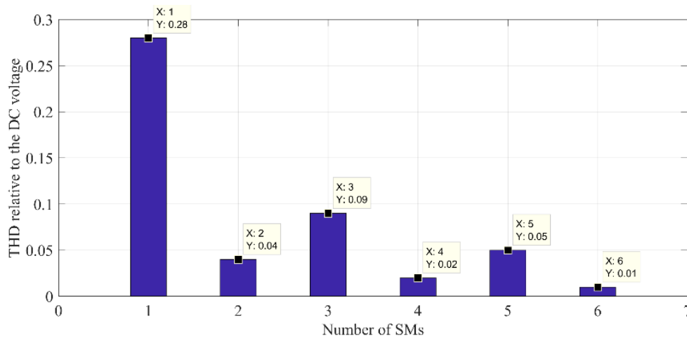
Fig. 7 The total harmonic distortion relative to DC component for different number of SM
