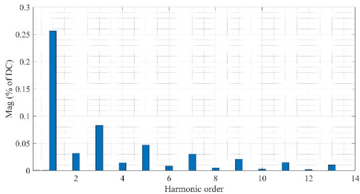
Fig. 3 FFT analysis of the typical output voltage waveform under load condition
