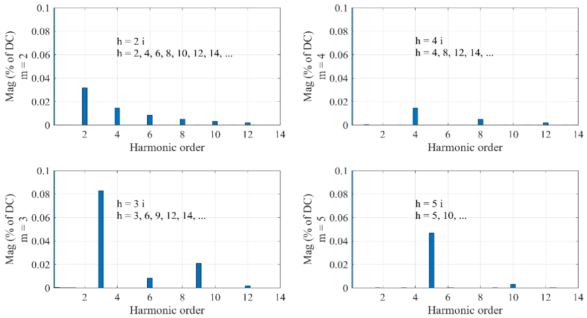
Fig. 6 FFT analysis of the generator output voltages (m = 2, 3, 4 & 5)
