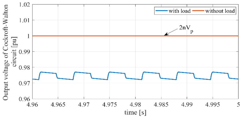
Fig. 2 The typical steady state output voltage waveform under load and no-load conditions
