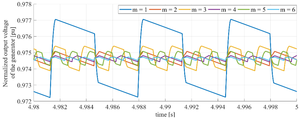
Fig. 5 Steady state normalized output voltages from the proposed generator for different number of SMs
