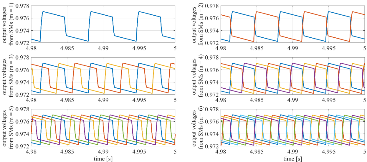
Fig. 4 Steady state SM voltages for different number of SMs
