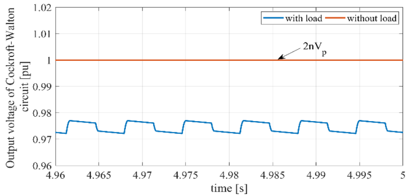
Fig. 2 The typical steady state output voltage waveform under load and no-load conditions
