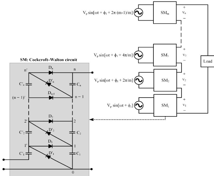
Fig. 1 Layout of the proposed modular HVDC generator with embedded Cockcroft-Walton circuits
