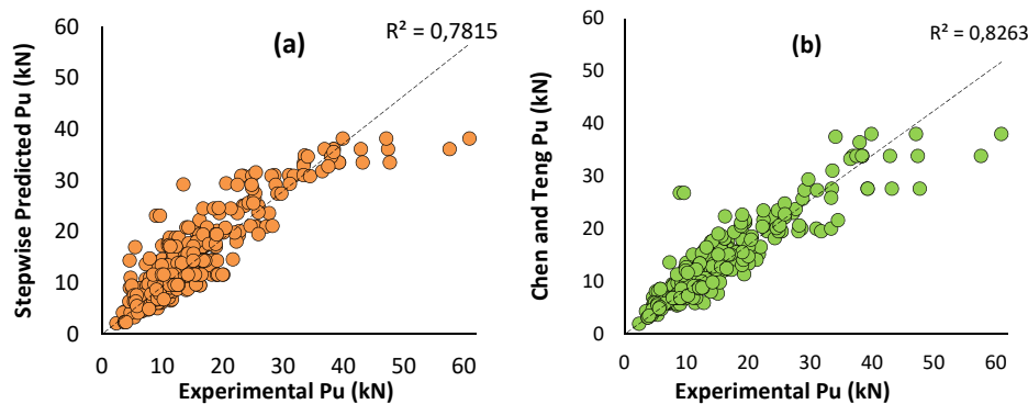
Fig. 3 Concrete pull-out tests (446 specimens), P_u predicted by: (a) Stepwise Regression Analysis; (b) Chen and Tengs' Model
