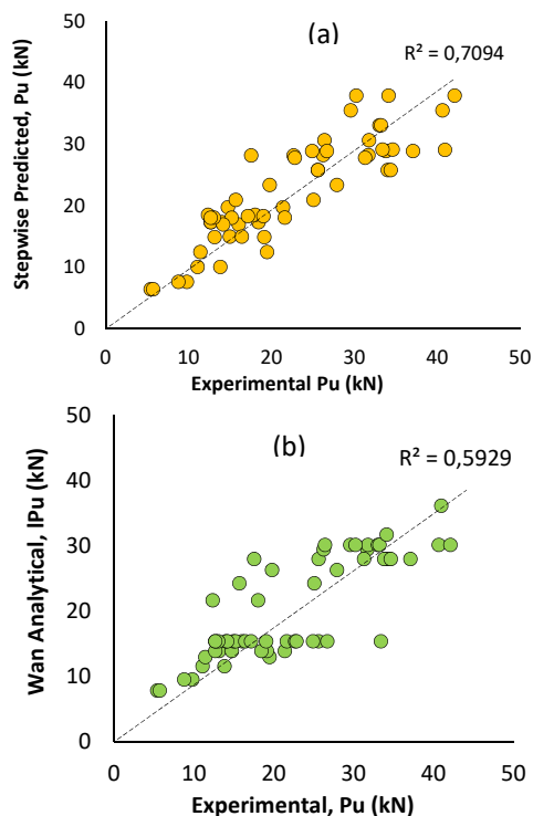
Fig. 4 Wan [13], P_u predicted by: (a) Stepwise Regression Analysis; (b) Wan's Model
