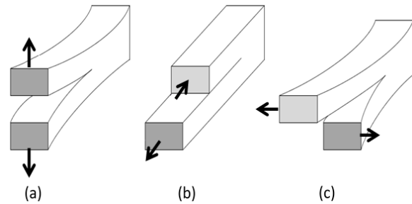
Fig. 1 Three fracture modes: (a) tensile or the opening (mode I), (b) in-plane shear or sliding (mode II) and (c) out-of-plane shear or tearing (mode III) [18]
