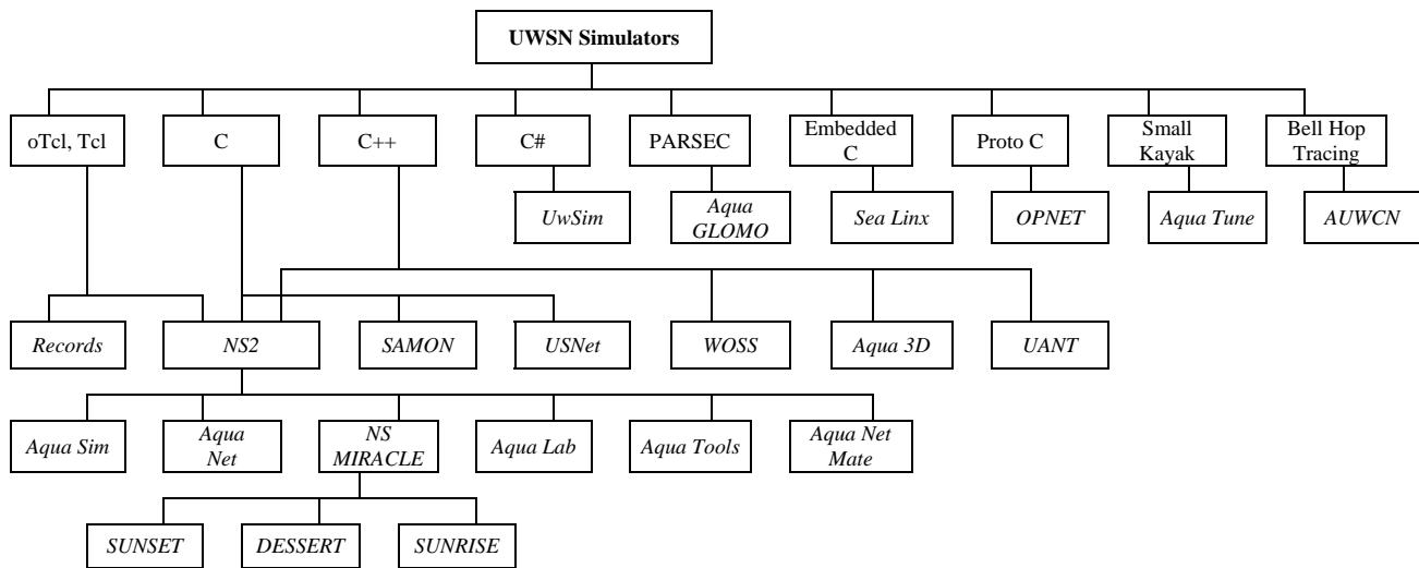
Fig. 2 UWSN Taxonomy
