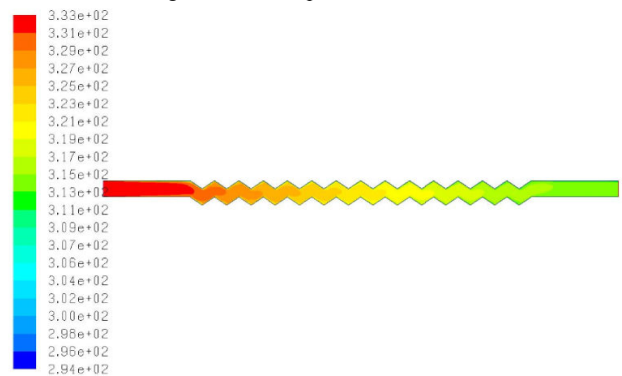
Fig. 25 Static temperature at Re 1400
