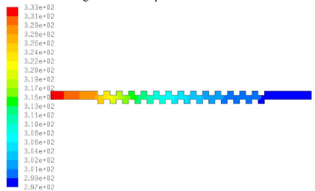
Fig. 51 Static temperature at Re 1400
