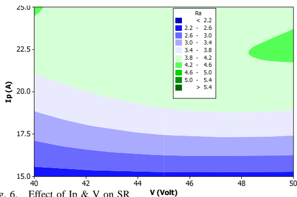
Fig. 6. Effect of Ip &amp; V on SR
