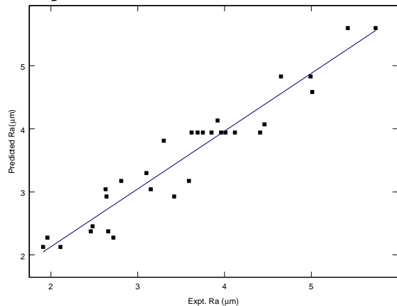
Fig. 1. Predicted vs. experimental SR
