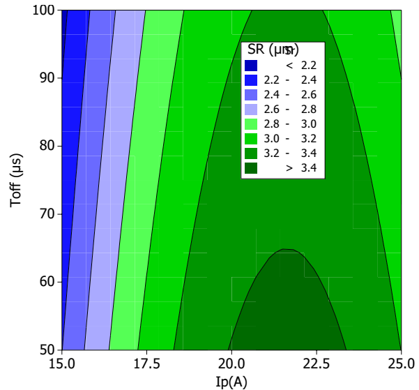
Fig. 4. Effect of I_p & T_{off} on SR
