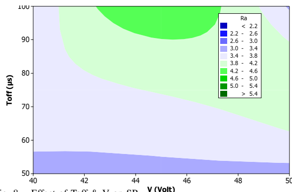
Fig. 8. Effect of Toff &amp; V on SR
