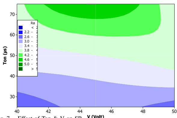
Fig. 7. Effect of Ton &amp; V on SR
