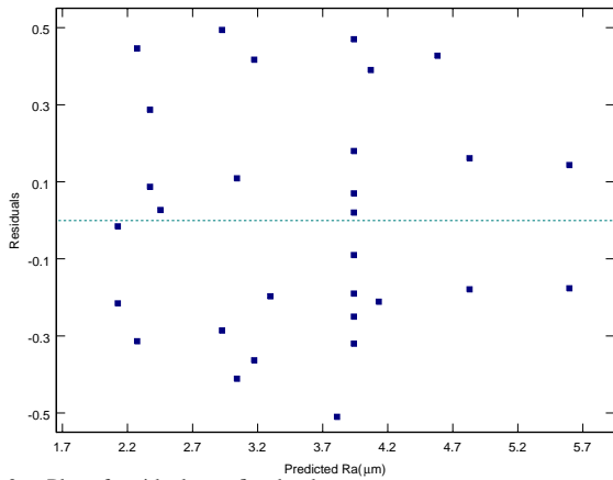
Fig. 2. Plot of residuals vs. fitted value
