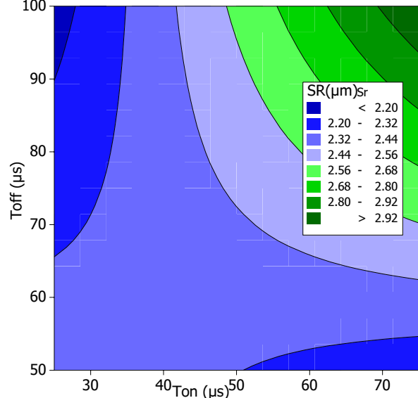
Fig. 5. Effect of T_{on} & T_{off} on SR
