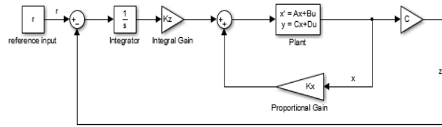
Fig. 2 LQR with integral action
