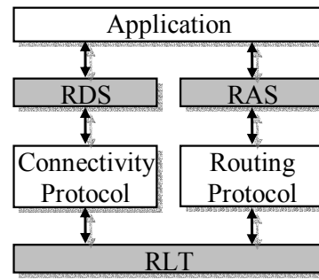
Fig 1: MASGRID Architecture
