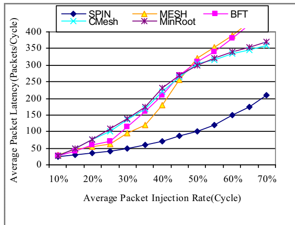
Fig. 11. Network latency under localized traffic(local factor=0.8) (poisson).
