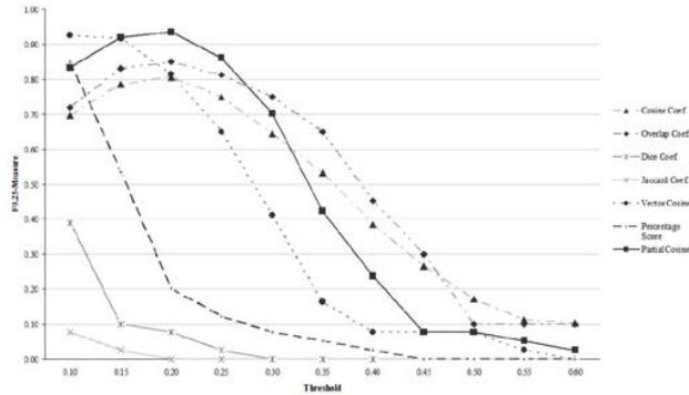
Fig. 5 similarity results for English
