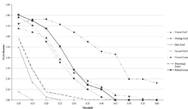
Fig. 6 similarity results for Japanese
