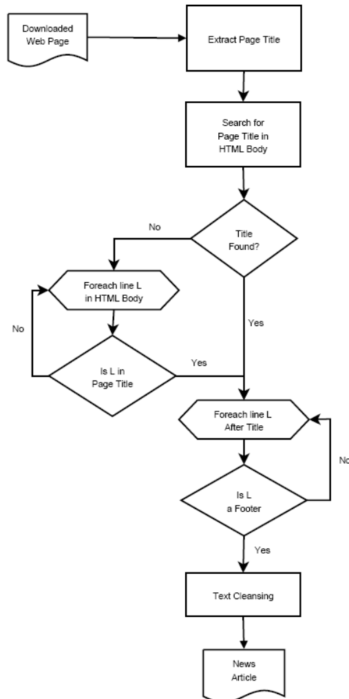
Fig. 3 overview of rule based extraction
